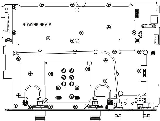
Figure 4-11. Main PCB and Connector Panel for 8 GHz Option
