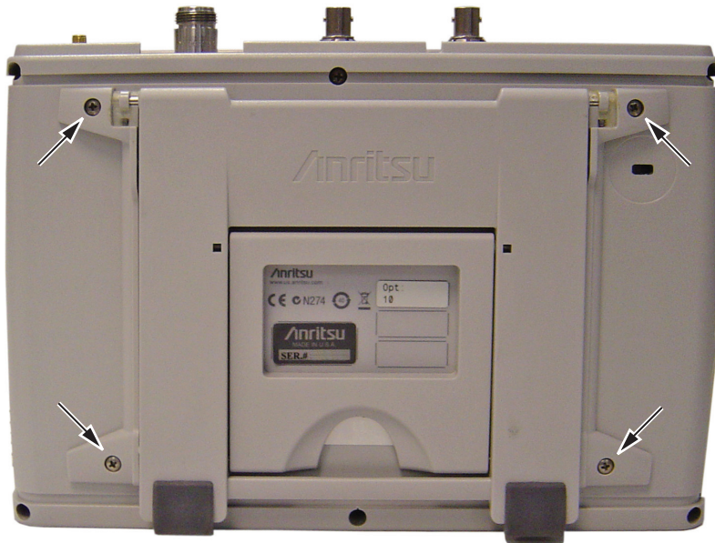
Figure 4-14. Remove the Four Screws to Replace the Tilt Bail
